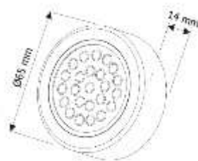
Surface-mounted dimensions
