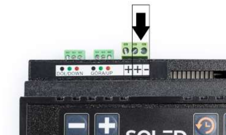
Figure 7 – Power supply connection points
