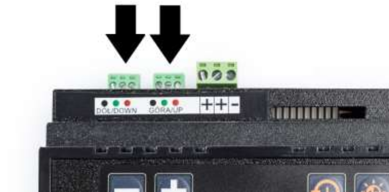
Figure 6 – Up and down sensor connection points
